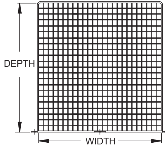
STI-9646 & STI-9647 Side View
