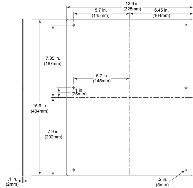
BACKPLATE STI-MBP1316
